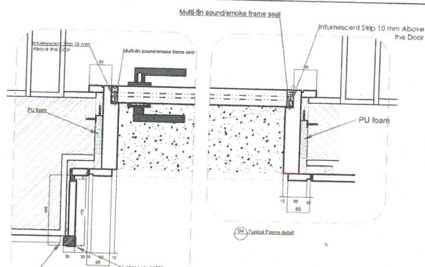
D4 Typical Frame detail
